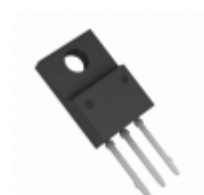
BA17812CP-E2 LAPIS Semiconductor IC REG LDO 12V 1A TO220CP-3
