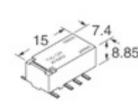
TX2SA-3V-1 Panasonic Electric Works RELAY GEN PURPOSE DPDT 1A 3V
