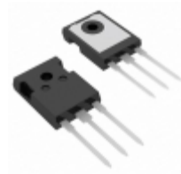
IXGH24N170A IXYS IGBT 1700V 24A 250W TO247AD
