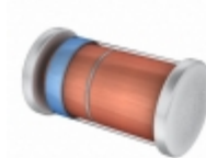
CLL4752A TR Central Semiconductor Corp DIODE ZENER 33V 1W MELF
