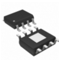
MIC5283-3.3YME-TR Microchip Technology IC REG LDO 3.3V 0.15A 8SOIC
