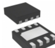
AP7361C-28FGE-7 Diodes Incorporated IC REG LDO 2.8V 1A U-DFN3030-8
