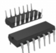
MCP42100-I/P Microchip Technology IC POT DGTL 100K 2CH SPI 14-DIP
