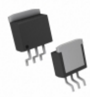
CS5205-1GDPR3 ON Semiconductor IC REG LDO ADJ 5A D2PAK
