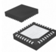
PIC24EP32GP202T-E/MM Microchip Technology IC MCU 16BIT 32KB FLASH 28QFN
