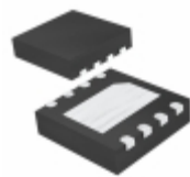
MAX5394NATA+T Maxim Integrated IC DGTL POT 256POS 100KOHM 8TDFN
