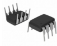
MAX539AEPA Maxim Integrated IC DAC SERIAL 5V LP 12BIT 8-DIP
