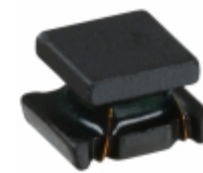
LQH32MN100K23L Murata Electronics North America FIXED IND 10UH 190MA 1.8 OHM SMD
