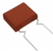
ECW-F2105HAQ Panasonic Electronic Components CAP FILM 1UF 3% 250VDC RADIAL
