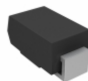
TPSMA43HE3/5AT Electro-Films (EFI) / Vishay TVS DIODE 34.8V 61.9V DO214AC
