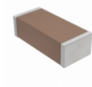
CGA7F1C0G3F120K085KA TDK Corporation CAP CER 12PF 3KV COG 1808
