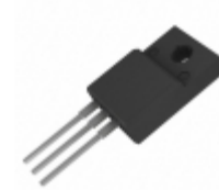
AOTF11S60L Alpha & Omega Semiconductor Inc. MOSFET N-CH 600V 11A TO220F
