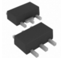
RT9069-33GX5 Richtek USA Inc. IC REG LDO 3.3V 0.2A SOT89-5
