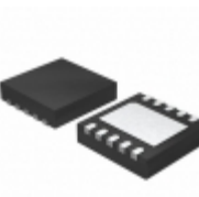
MCP4262T-103E/MF Microchip Technology IC POT DGTL DUAL 10K RHEO 10DFN
