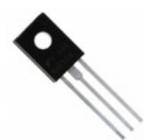
BD442S AMI Semiconductor / ON Semiconductor TRANS PNP 80V 4A TO-126
