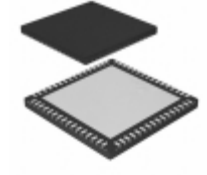
AT32UC3B0128AU-Z2UR Micrel / Microchip Technology IC MCU 32BIT 128KB FLASH 64QFN
