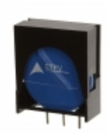
B72220T2381K101 EPCOS (TDK) VARISTOR 620V 10KA 3SIP
