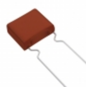
ECW-F2W154JAQ Panasonic Electronic Components CAP FILM 0.15UF 5% 450VDC RADIAL
