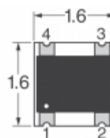
EHF-FD1541 Panasonic Electronic Components DIRECTIONAL COUPLER 1850MHZ-14DB
