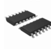
AD8625ARZ-REEL Analog Devices Inc. IC OPAMP JFET 5MHZ RRO 14SOIC
