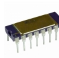
AD524BDZ Analog Devices Inc. IC OPAMP INSTR 1MHZ 16CDIP
