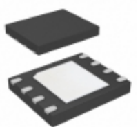
SST26VF064BT-104I/MN Microchip Technology IC FLASH 64MBIT 104MHZ 8WDFN
