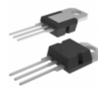
MIC2940A-12BT Microchip Technology IC REG LDO 12V 1.25A TO220-3
