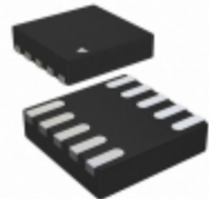
MIC5313-F5YMT-TR Microchip Technology IC REG LDO 1.5V/1.3V 0.3A 10TMLF
