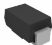
SS15-M3/61T Vishay Semiconductor Diodes Division DIODE SCHOTTKY 1A 50V DO- 214AC
