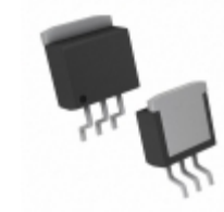
MIC39300-2.5WU-TR Microchip Technology IC REG LDO 2.5V 3A TO263-3
