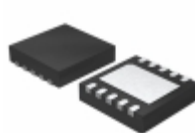
AD7686BCPZRL7 Analog Devices Inc. IC ADC 16BIT 500KSPS 10-LFCSP
