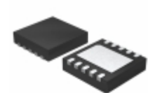
AD7687BCPZ-R2 Analog Devices Inc. IC ADC 16BIT SAR 250KSPS 10LFCSP
