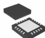
MCP4361-502E/ML Microchip Technology IC POT 8BIT QUAD 5K 20QFN
