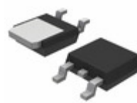
NJVMJD340T4G-VF01 ON Semiconductor TRANS NPN 300V 0.5A DPAK-4
