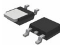
NJVMJD44E3T4G ON Semiconductor TRANS NPN DARL 80V 10A DPAK-4
