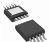
LTC2634HMSE-LZ8#PBF ADI (Analog Devices, Inc.) IC DAC 8BIT QUAD 2.5V 10MSOP
