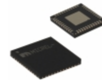
SY89112UMG Microchip Technology IC CLK BUFFER 2:12 3GHZ 44MLF
