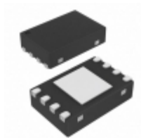
93LC66BT-I/MNY Microchip Technology IC EEPROM 4KBIT 2MHZ 8TDFN
