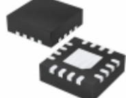
MCP4631T-503E/ML Microchip Technology IC DGTL POT 50K 129TAPS 16-QFN
