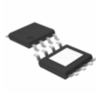
BD00FC0WEFJ-E2 Rohm Semiconductor IC REG LDO ADJ 1A 8HTSOPJ
