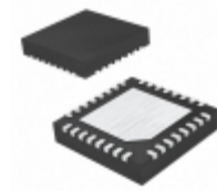
DSPIC33EP32MC502-H/MM Microchip Technology IC MCU 16BIT 32KB FLASH 28QFN
