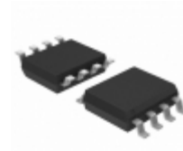
MIC39101-1.8BM-TR Microchip Technology IC REG LDO 1.8V 1A 8SOIC
