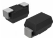
SMAJ33A Bourns Inc. TVS DIODE 33VWM 53.3VC DO214AC
