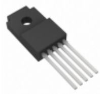
BA08CC0WT Rohm Semiconductor IC REG LDO 8V 1A TO220FP-5
