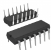
MCP4261-503E/P Microchip Technology IC DGTL POT 50K 2CH 14DIP
