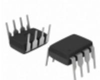
AT25020-10PI-2.7 Microchip Technology IC EEPROM 2KBIT 2.1MHZ 8DIP
