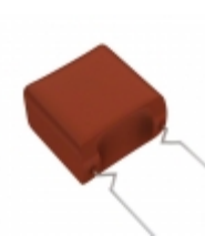
ECW-F2565JAQ Panasonic Electronic Components CAP FILM 5.6UF 5% 250VDC RADIAL
