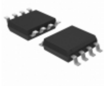
SY100EL05ZI-TR Microchip Technology IC GATE AND/NAND DIFF 2INP 8SOIC
