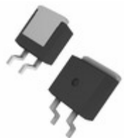
IXFA26N50P3 IXYS MOSFET N-CH 500V 26A TO-263AA
