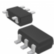
XC6121A418MR-G Torex Semiconductor Ltd IC WATCHDOG TIMER SOT-25
