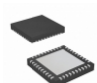
PIC16LF18876-E/MV Microchip Technology IC MCU 8BIT 28KB FLASH 40UQFN
