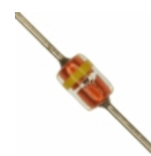
MTZJT-722.2B Rohm Semiconductor DIODE ZENER 2.2V 500MW DO34
