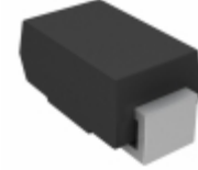
SMBZ5941B-E3/52 Vishay / Semiconductor - Diodes Division DIODE ZENER 47V 3W DO214AA
